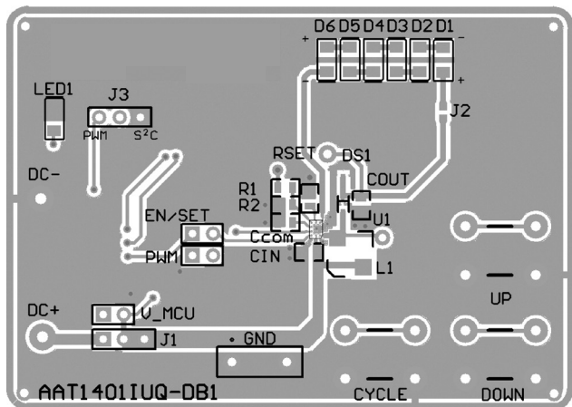
Figure 7: AAT1401 Evaluation Board Top Side Layout.
